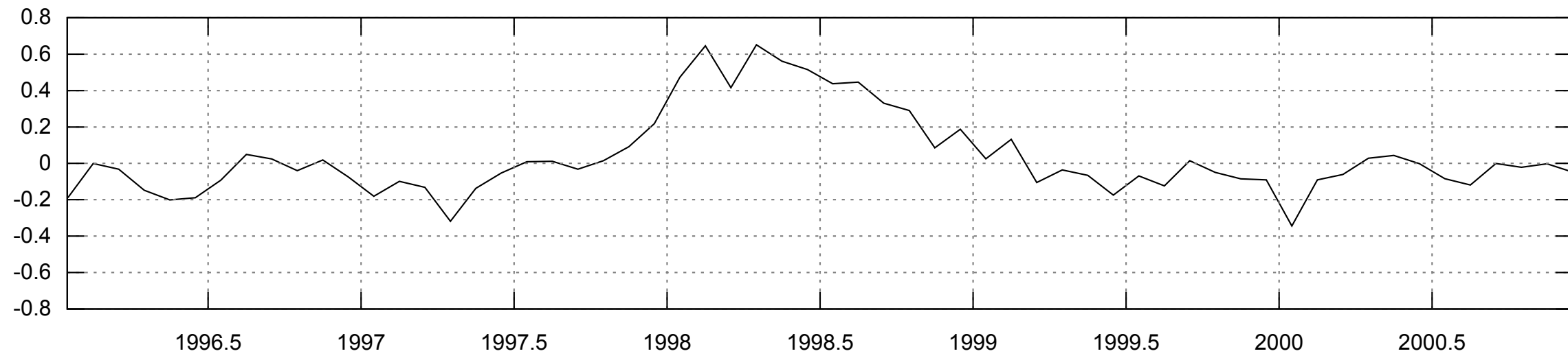
global mean
