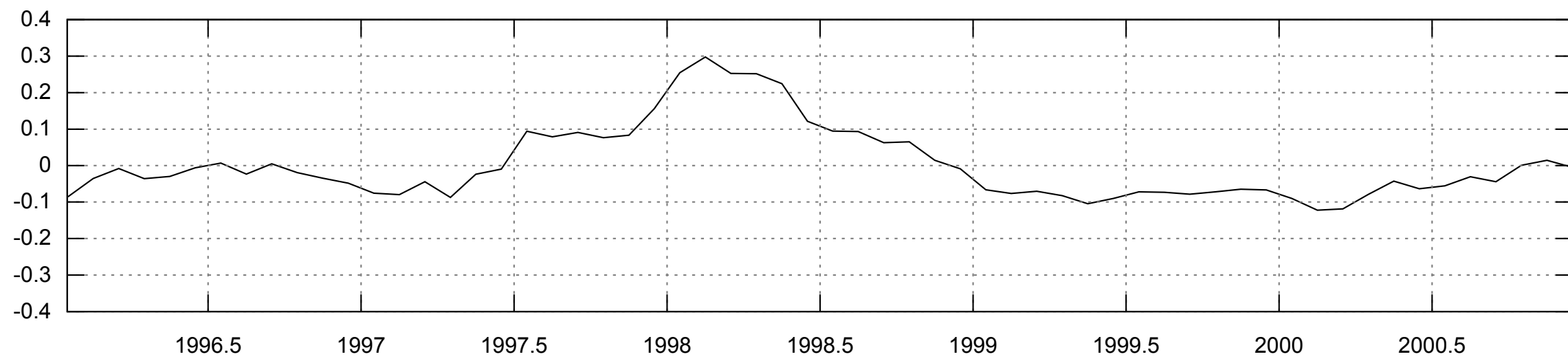
tropical mean
